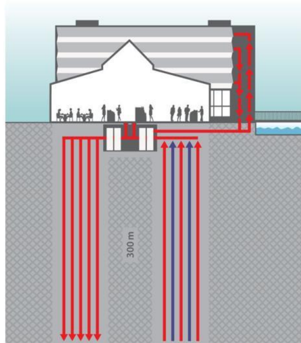
Heating or cooling extracted from geo-wells
